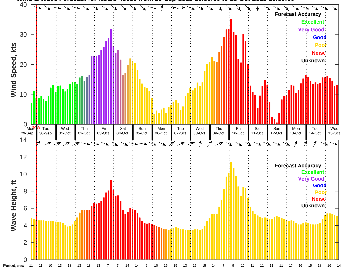
Wind & Wave Forecast for NDBC 46069 from 29-Sep-2025 16:00:00 to 15-Oct-2025 16:00:00
