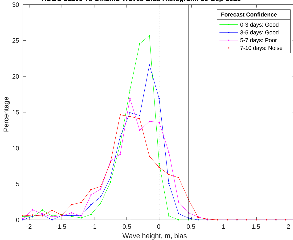
NDBC 51209 vs CMEMS Waves Bias Histogram: 30-Sep-2025
