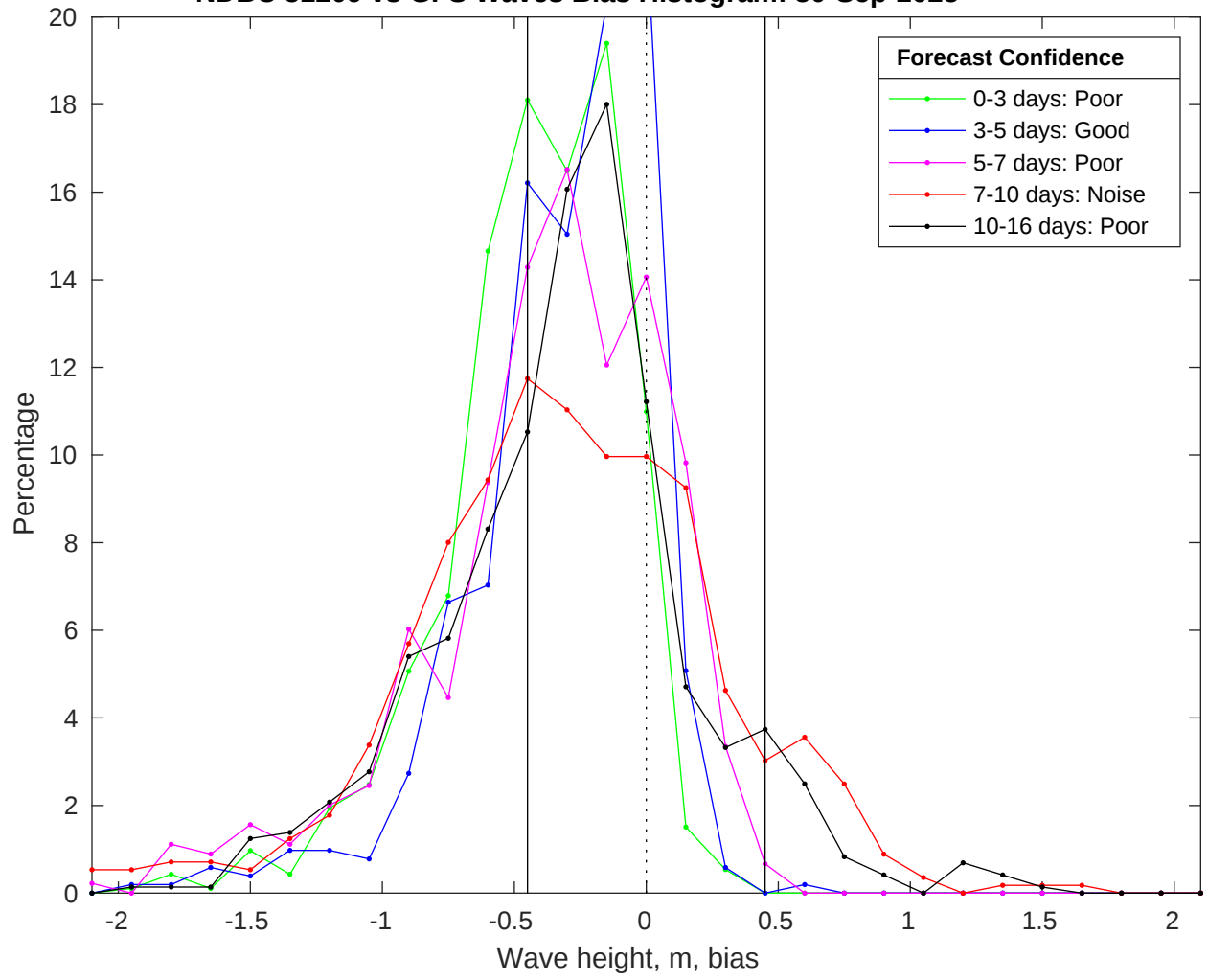
NDBC 51209 vs GFS Waves Bias Histogram: 30-Sep-2025
