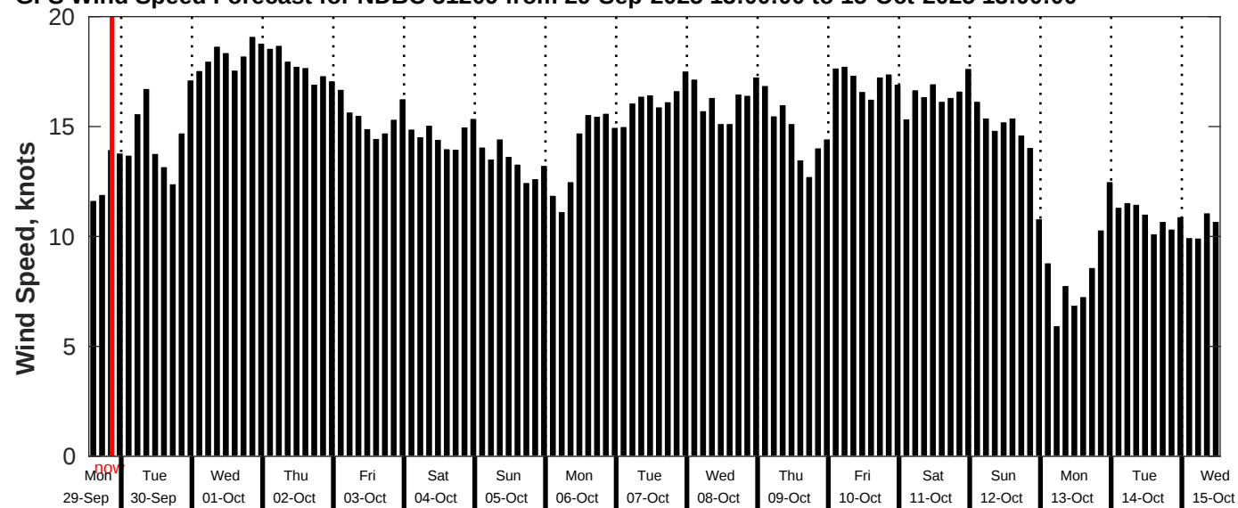
GFS Wind Speed Forecast for NDBC 51209 from 29-Sep-2025 13:00:00 to 15-Oct-2025 13:00:00
