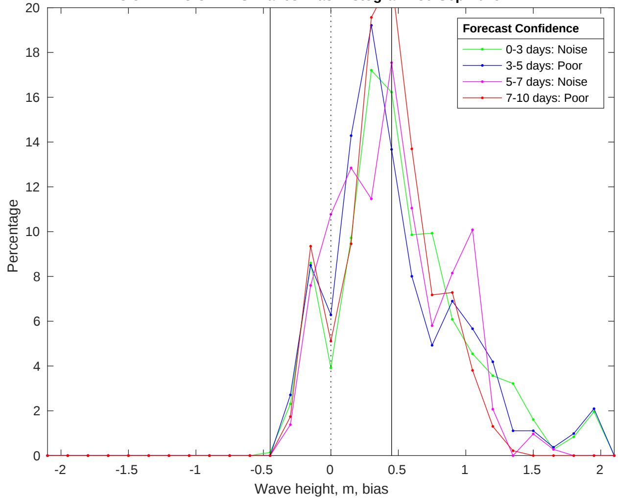
NDBC 51211 vs CMEMS Waves Bias Histogram: 30-Sep-2025
