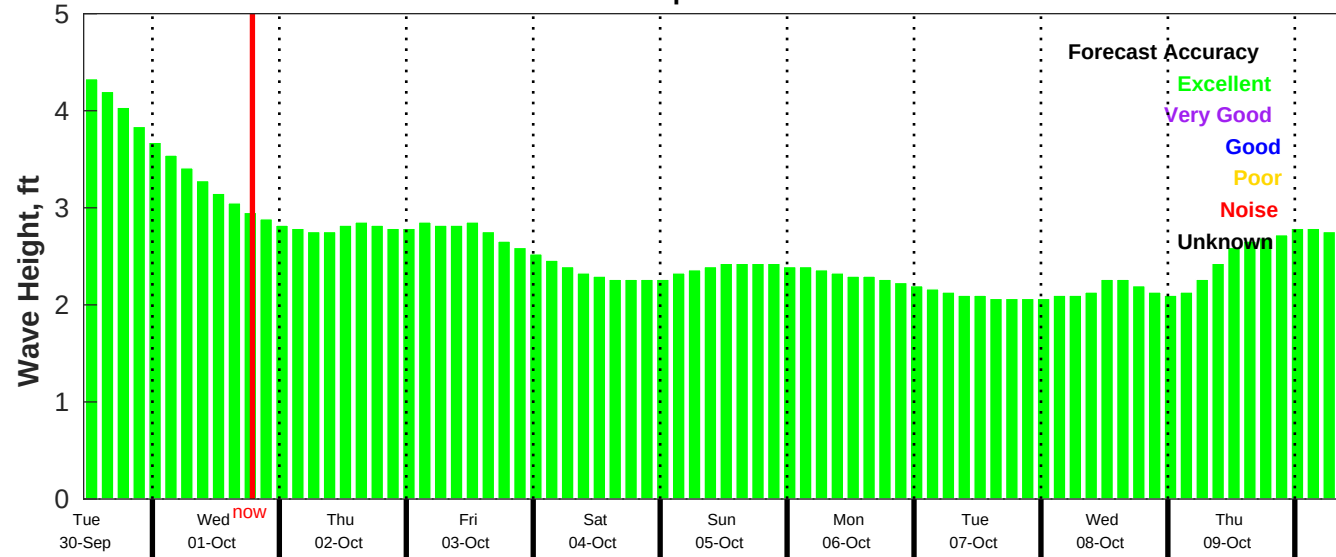
CMEMS Wave Forecast for NDBC 52211 from 29-Sep-2025 11:00:00 to 09-Oct-2025 11:00:00
