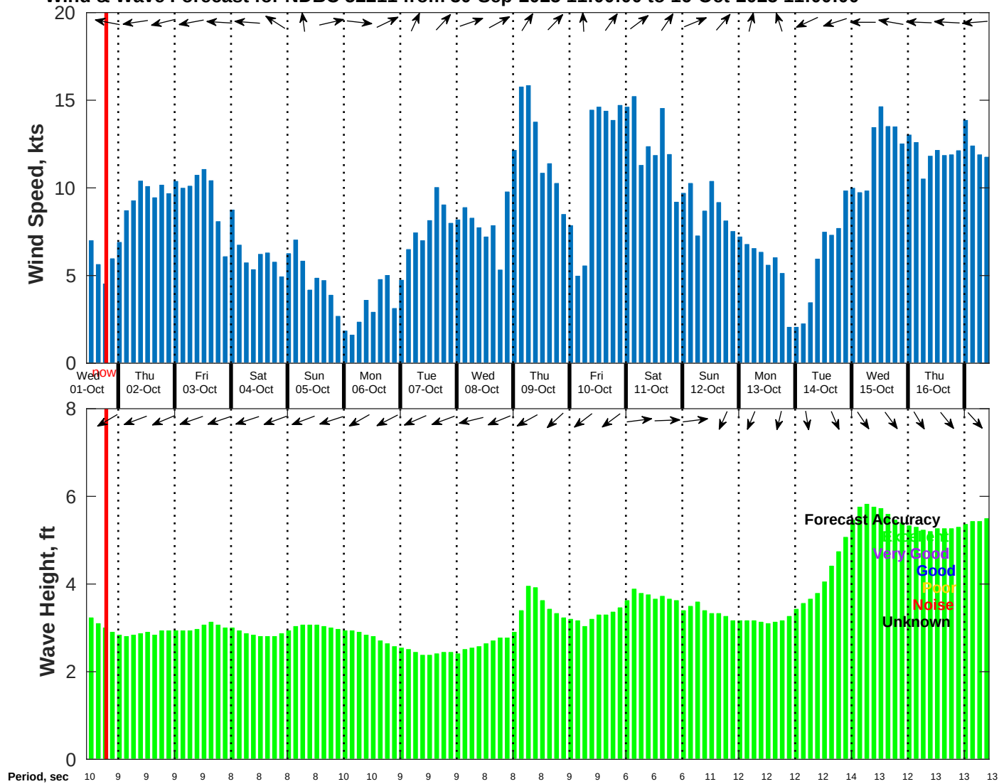
Wind & Wave Forecast for NDBC 52211 from 30-Sep-2025 11:00:00 to 16-Oct-2025 11:00:00
