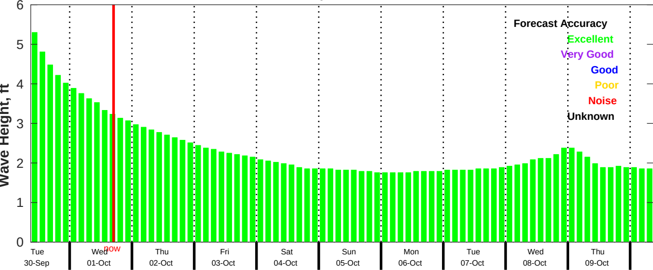
CMEMS Wave Forecast for NDBC 52212 from 29-Sep-2025 09:00:00 to 09-Oct-2025 09:00:00
