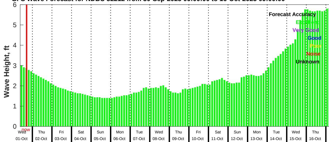
GFS Wave Forecast for NDBC 52212 from 30-Sep-2025 09:00:00 to 16-Oct-2025 09:00:00
