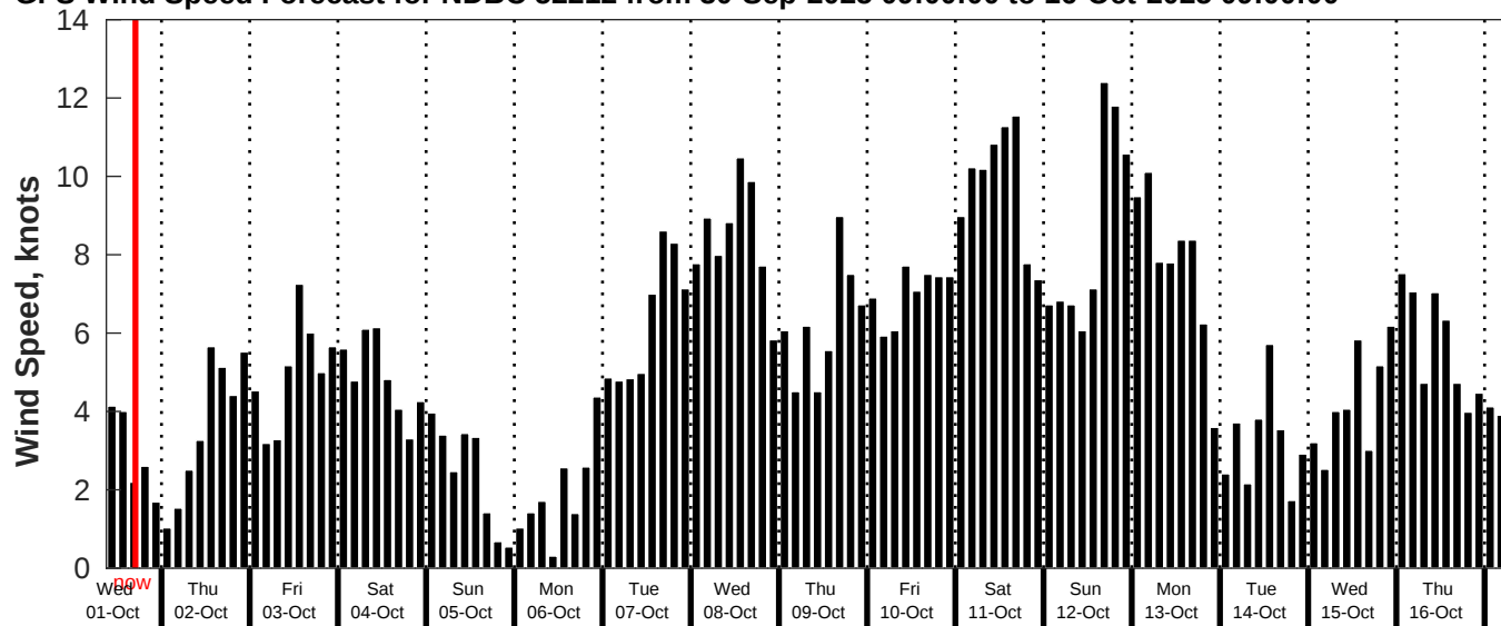
GFS Wind Speed Forecast for NDBC 52212 from 30-Sep-2025 09:00:00 to 16-Oct-2025 09:00:00
