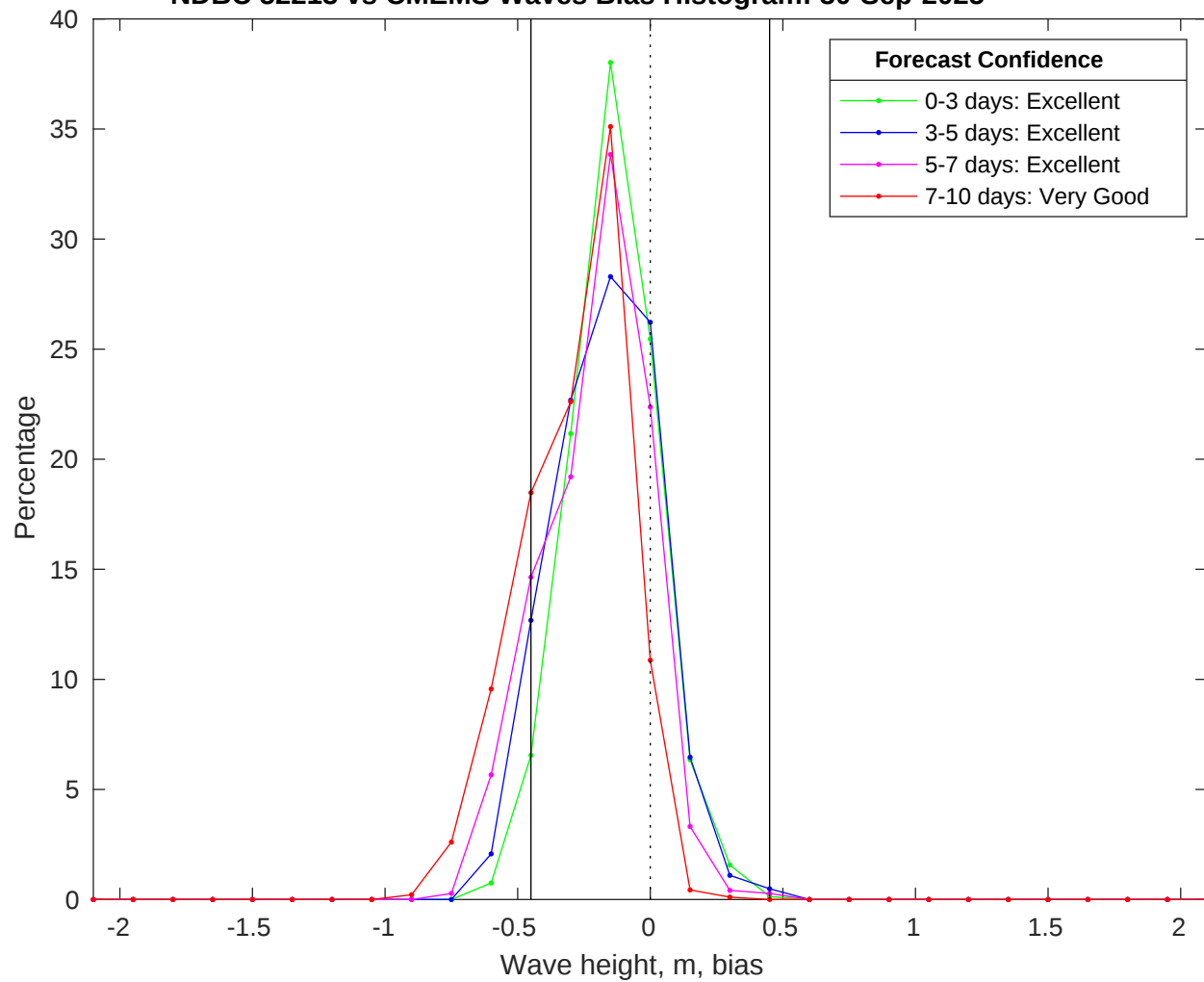
NDBC 52213 vs CMEMS Waves Bias Histogram: 30-Sep-2025
