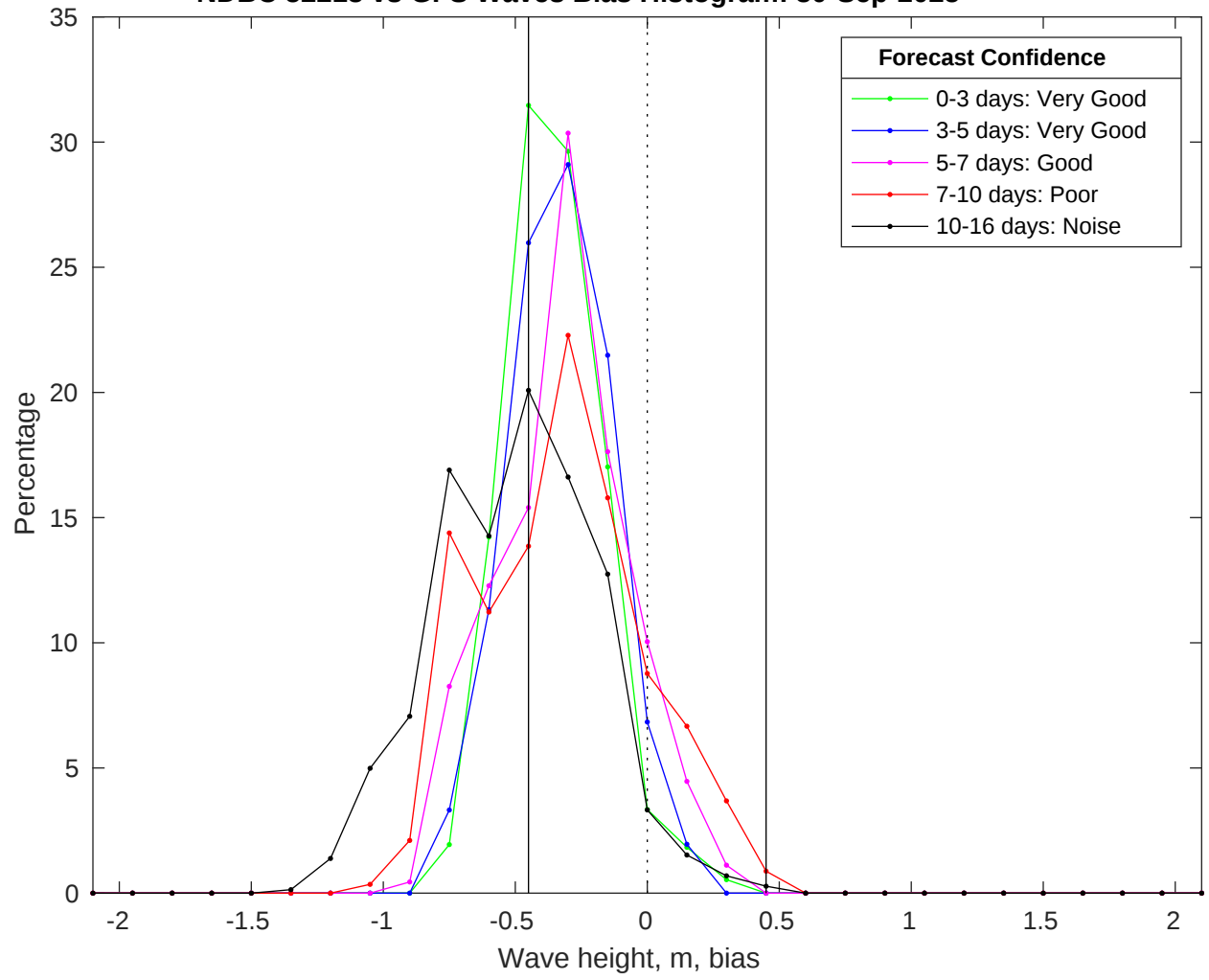
NDBC 52213 vs GFS Waves Bias Histogram: 30-Sep-2025
