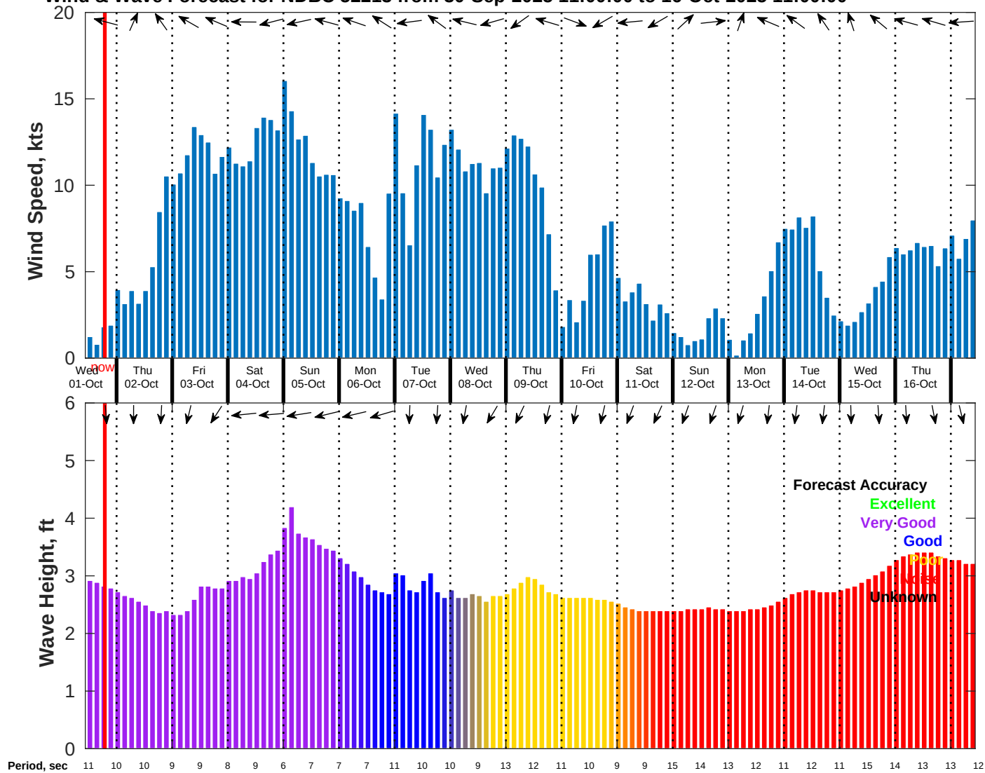
Wind & Wave Forecast for NDBC 52213 from 30-Sep-2025 11:00:00 to 16-Oct-2025 11:00:00
