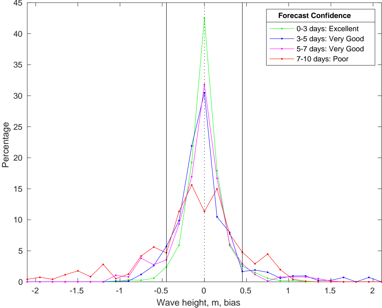
NDBC 41004 vs CMEMS Waves Bias Histogram: 01-Oct-2025
