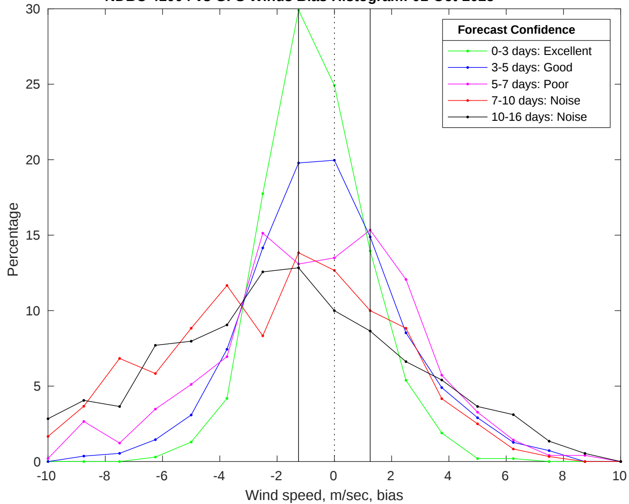
NDBC 41004 vs GFS Winds Bias Histogram: 01-Oct-2025
