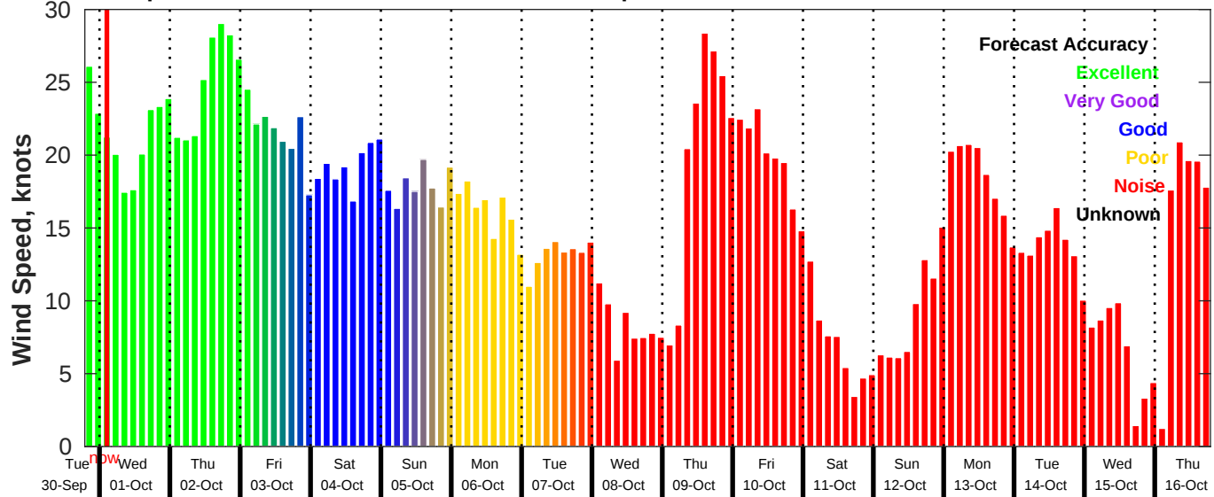
GFS Wind Speed Forecast for NDBC 41004 from 30-Sep-2025 19:00:00 to 16-Oct-2025 19:00:00
