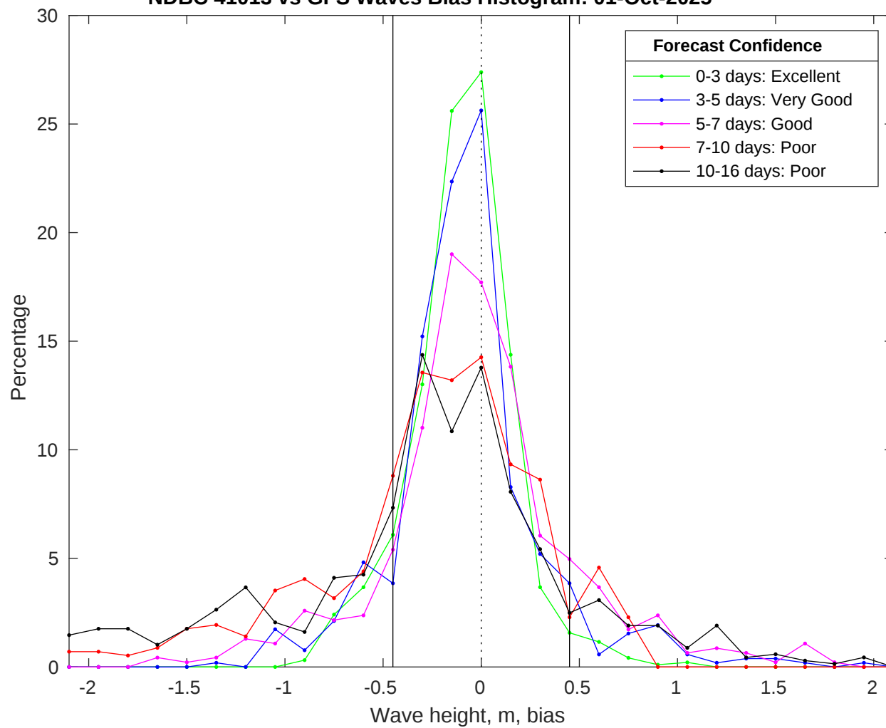
NDBC 41013 vs GFS Waves Bias Histogram: 01-Oct-2025
