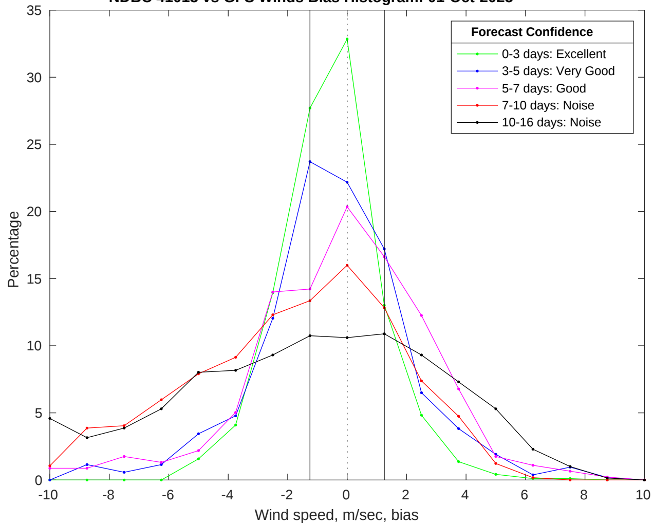
NDBC 41013 vs GFS Winds Bias Histogram: 01-Oct-2025
