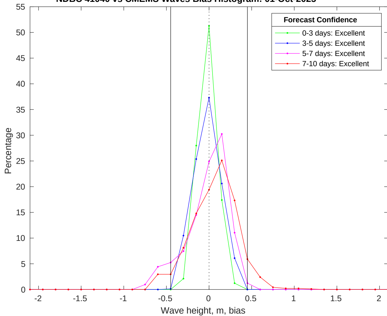
NDBC 41040 vs CMEMS Waves Bias Histogram: 01-Oct-2025
