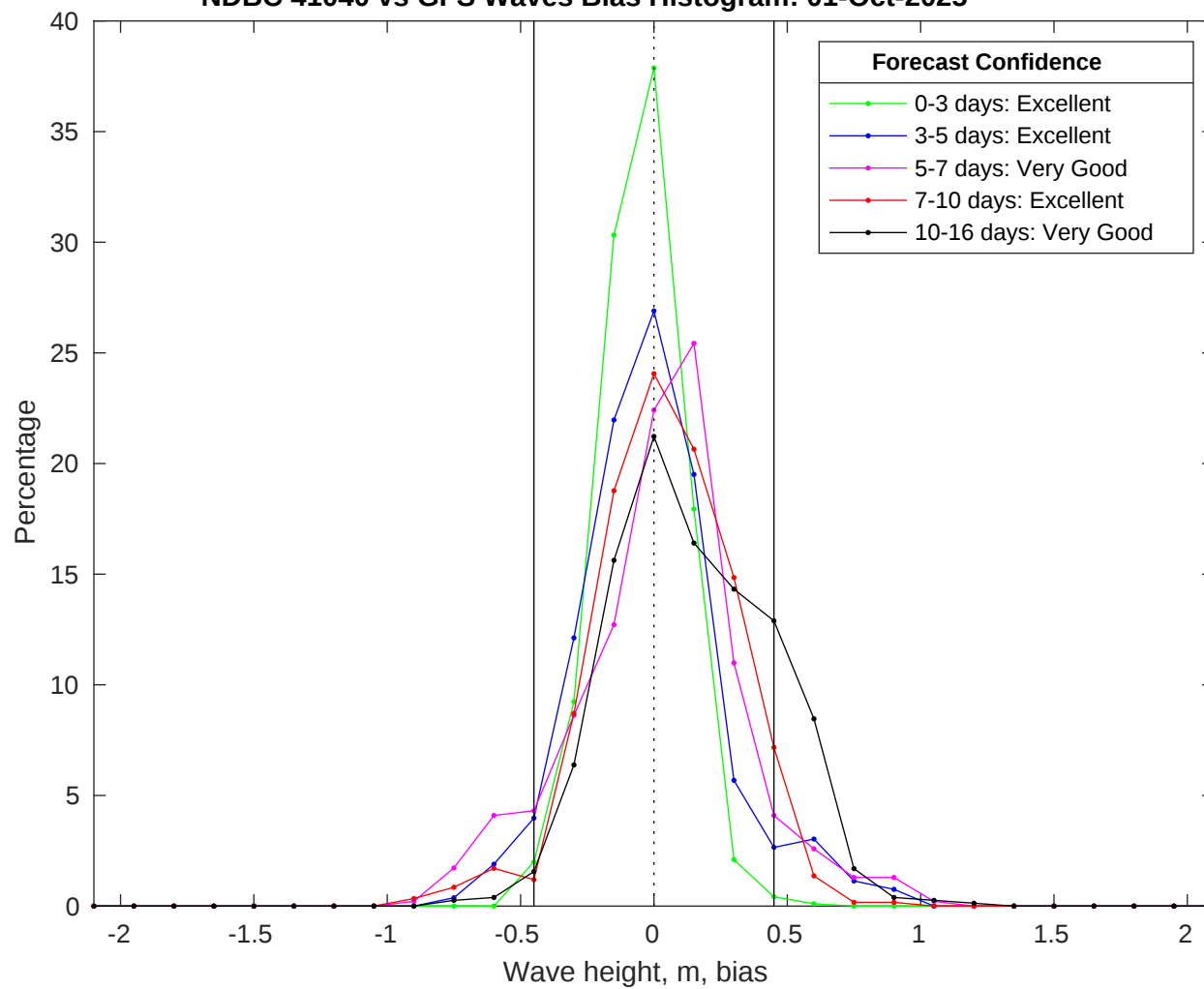
NDBC 41040 vs GFS Waves Bias Histogram: 01-Oct-2025
