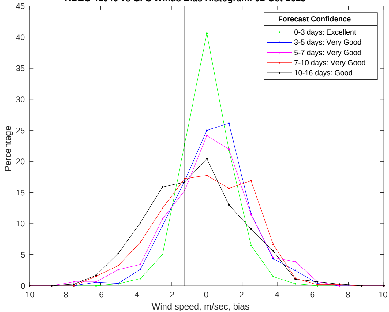
NDBC 41040 vs GFS Winds Bias Histogram: 01-Oct-2025
