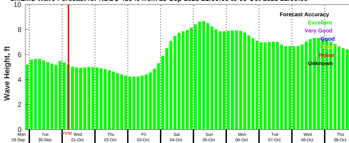
CMEMS Wave Forecast for NDBC 41040 from 29-Sep-2025 21:00:00 to 09-Oct-2025 21:00:00
