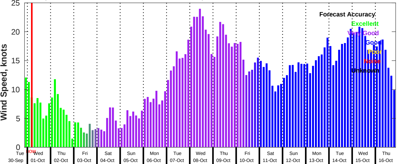
GFS Wind Speed Forecast for NDBC 41040 from 30-Sep-2025 21:00:00 to 16-Oct-2025 21:00:00
