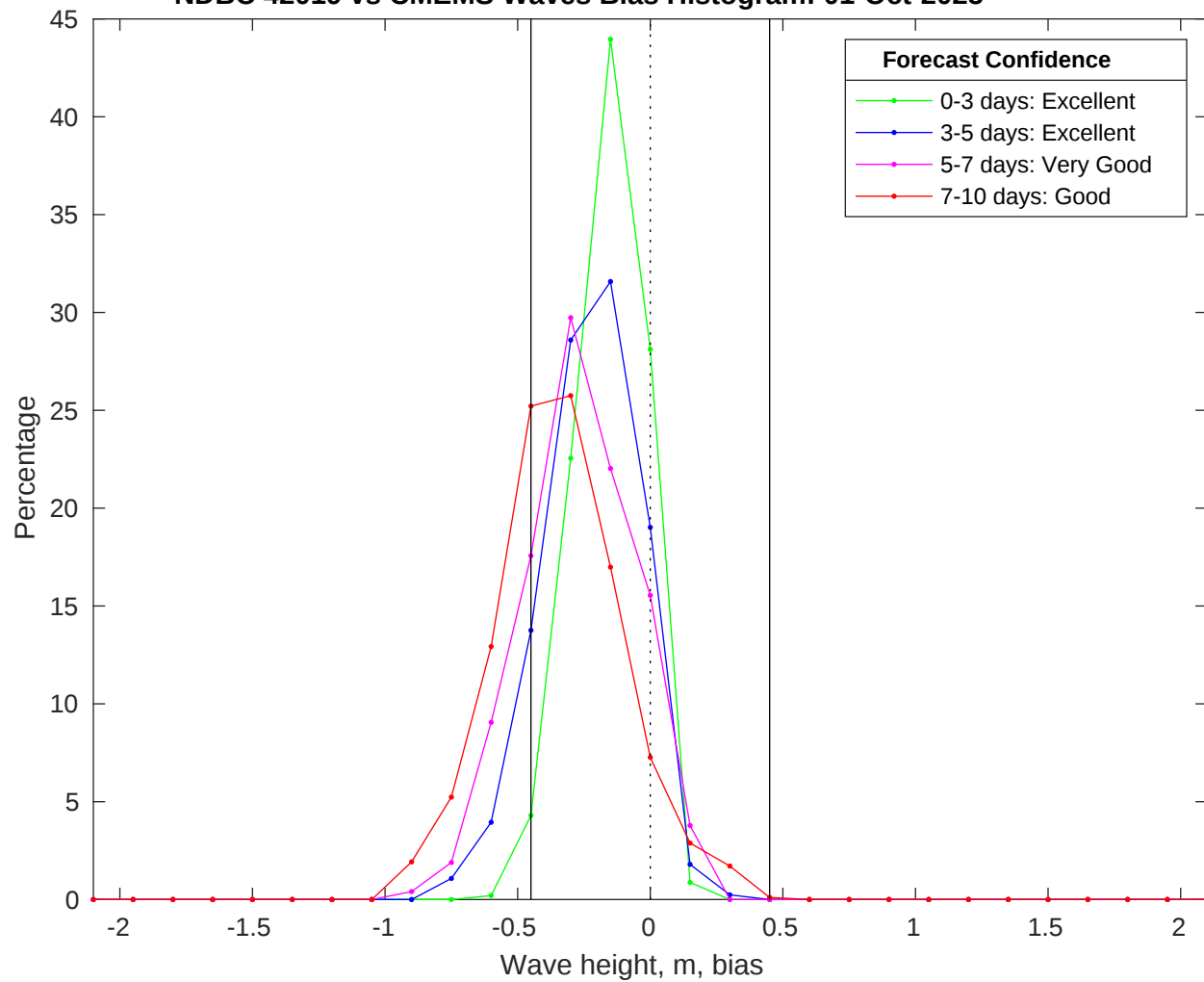
NDBC 42019 vs CMEMS Waves Bias Histogram: 01-Oct-2025
