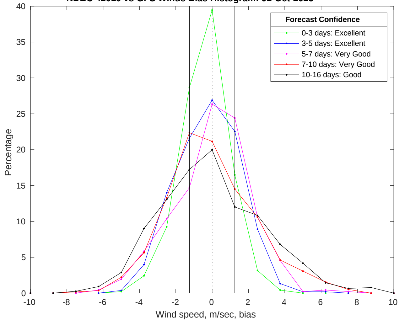
NDBC 42019 vs GFS Winds Bias Histogram: 01-Oct-2025
