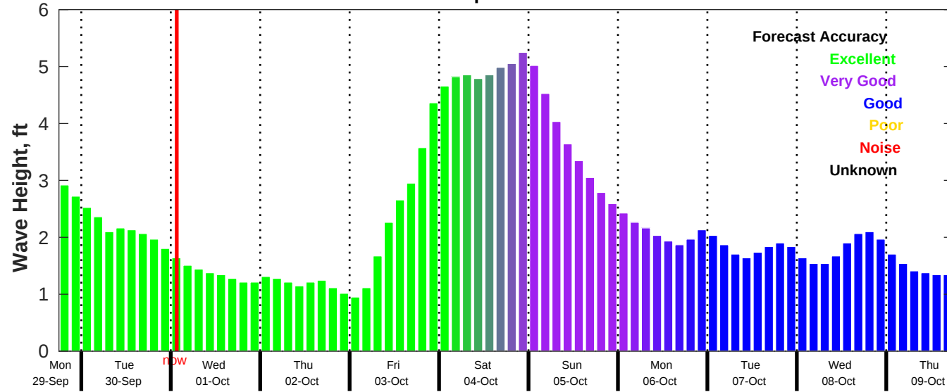
CMEMS Wave Forecast for NDBC 42019 from 29-Sep-2025 18:00:00 to 09-Oct-2025 18:00:00
