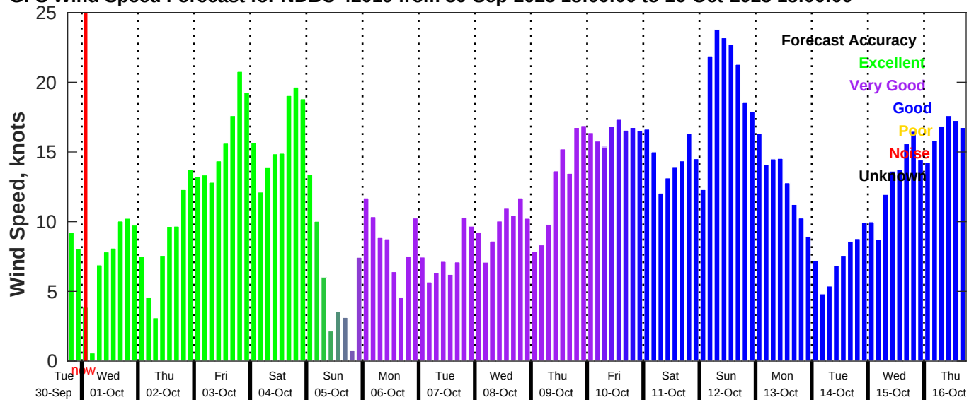
GFS Wind Speed Forecast for NDBC 42019 from 30-Sep-2025 18:00:00 to 16-Oct-2025 18:00:00
