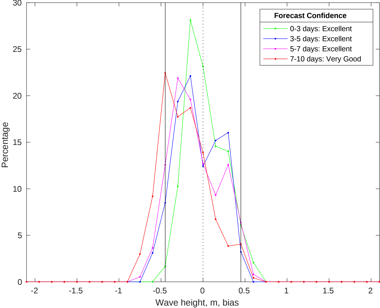
NDBC 42020 vs CMEMS Waves Bias Histogram: 01-Oct-2025
