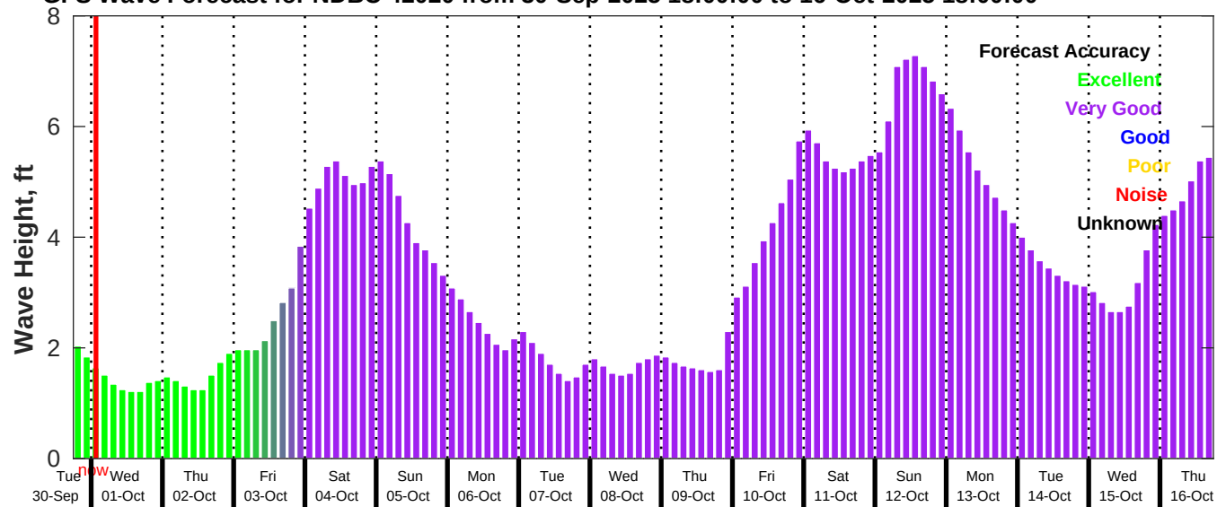
GFS Wave Forecast for NDBC 42020 from 30-Sep-2025 18:00:00 to 16-Oct-2025 18:00:00
