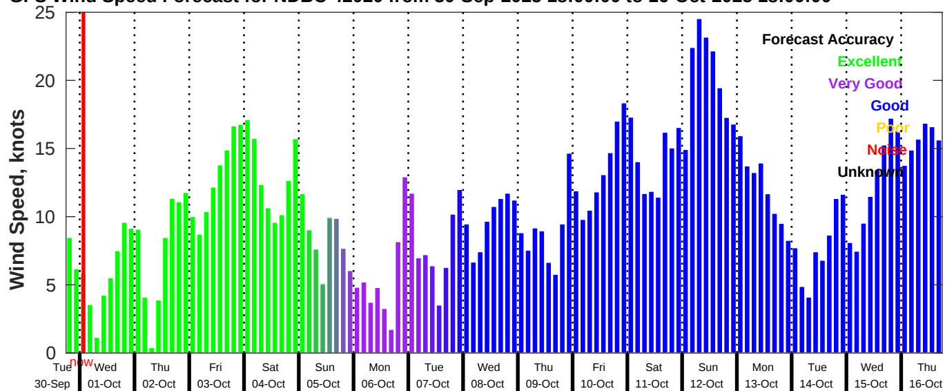
GFS Wind Speed Forecast for NDBC 42020 from 30-Sep-2025 18:00:00 to 16-Oct-2025 18:00:00
