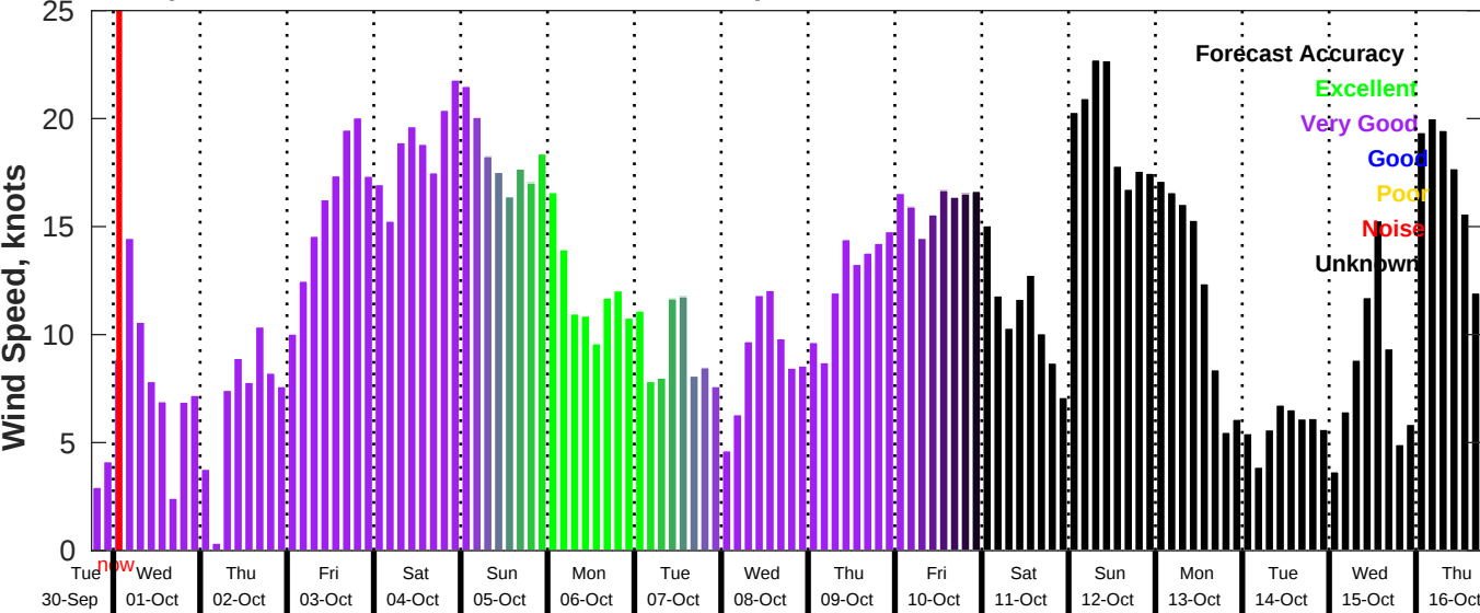
GFS Wind Speed Forecast for NDBC 42035 from 30-Sep-2025 18:00:00 to 16-Oct-2025 18:00:00
