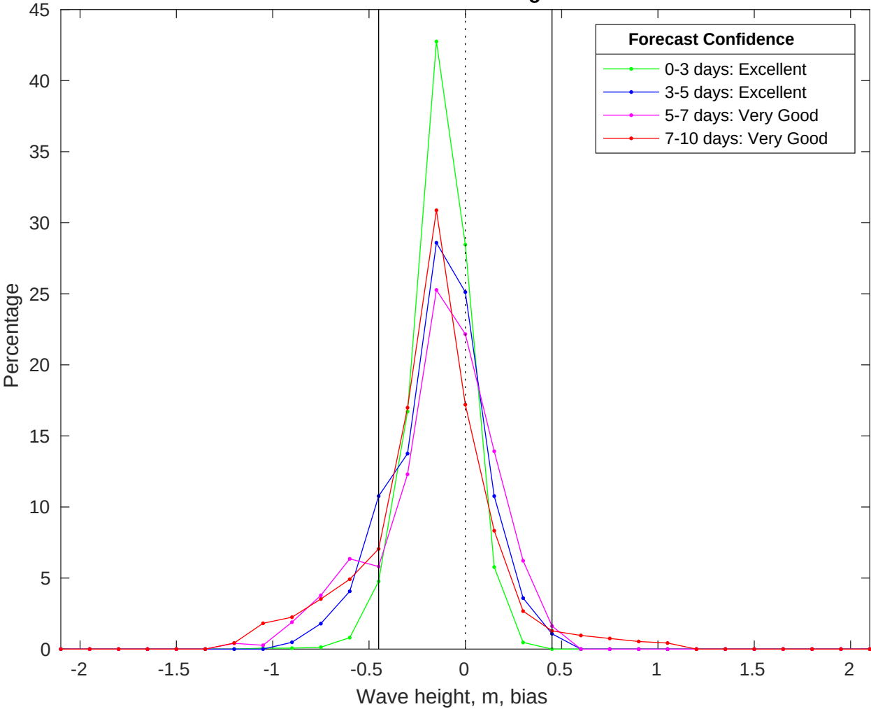
NDBC 42036 vs CMEMS Waves Bias Histogram: 01-Oct-2025
