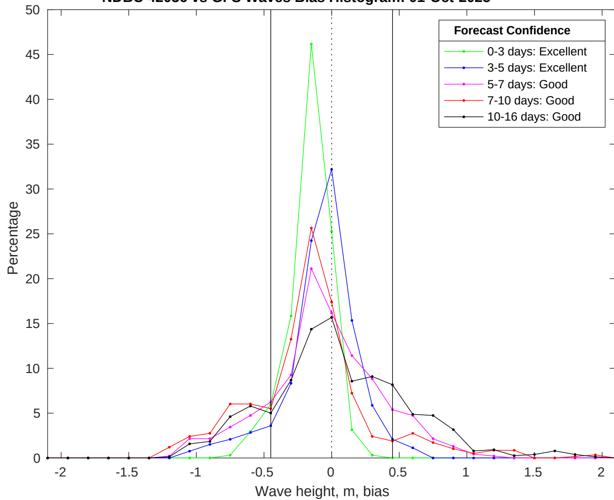
NDBC 42036 vs GFS Waves Bias Histogram: 01-Oct-2025
