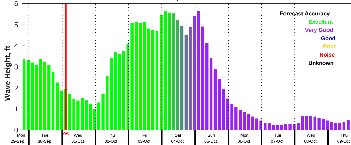
CMEMS Wave Forecast for NDBC 42036 from 29-Sep-2025 19:00:00 to 09-Oct-2025 19:00:00
