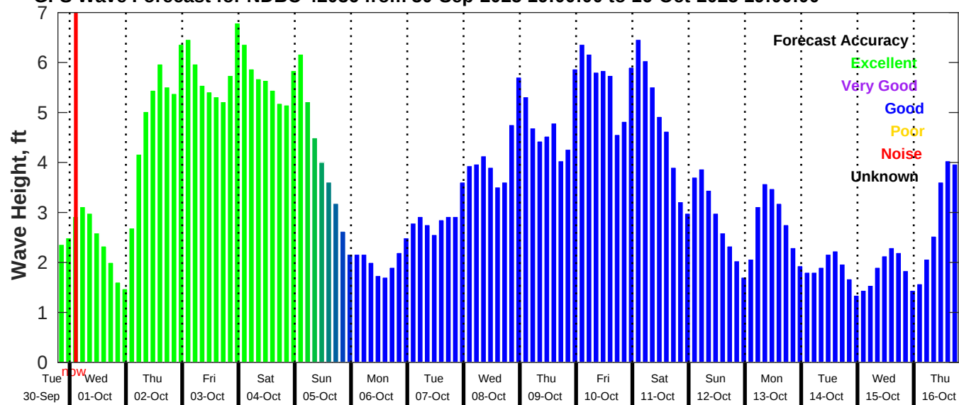
GFS Wave Forecast for NDBC 42036 from 30-Sep-2025 19:00:00 to 16-Oct-2025 19:00:00
