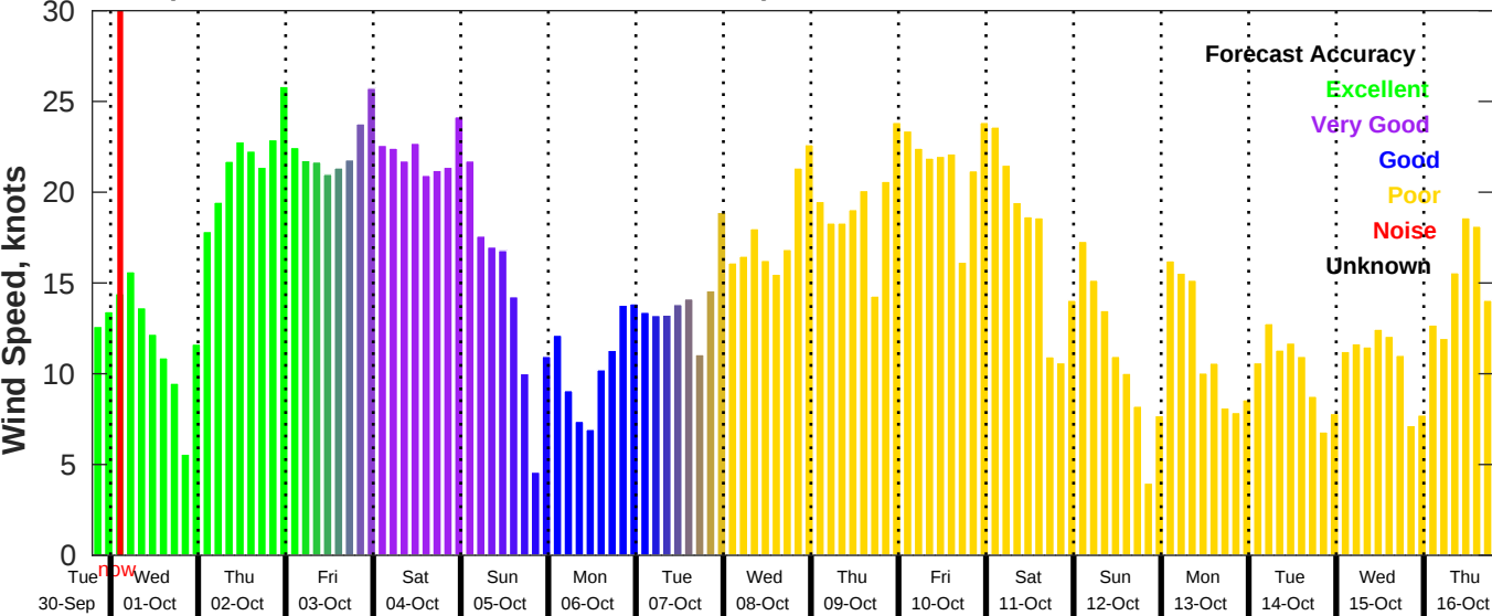
GFS Wind Speed Forecast for NDBC 42036 from 30-Sep-2025 19:00:00 to 16-Oct-2025 19:00:00
