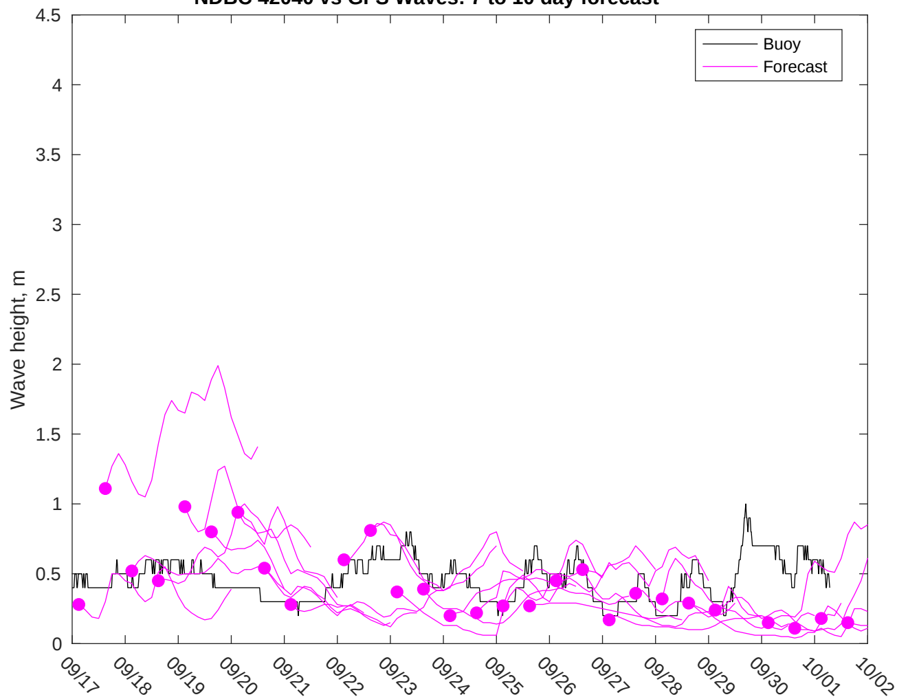
NDBC 42040 vs GFS Waves: 7 to 10 day forecast
