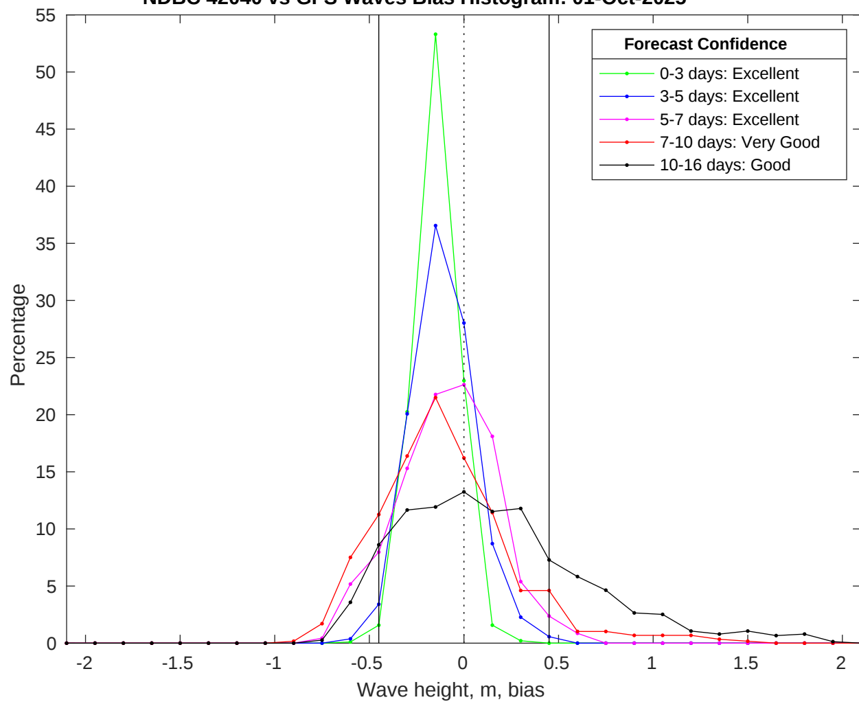
NDBC 42040 vs GFS Waves Bias Histogram: 01-Oct-2025
