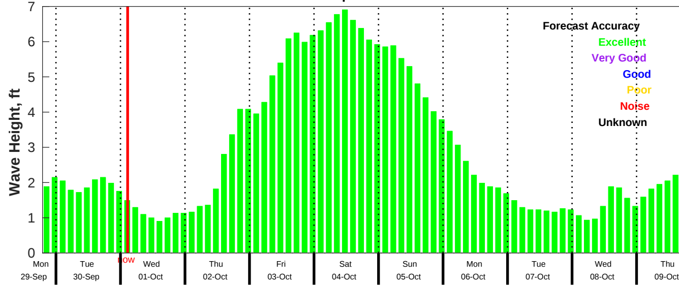
CMEMS Wave Forecast for NDBC 42040 from 29-Sep-2025 19:00:00 to 09-Oct-2025 19:00:00
