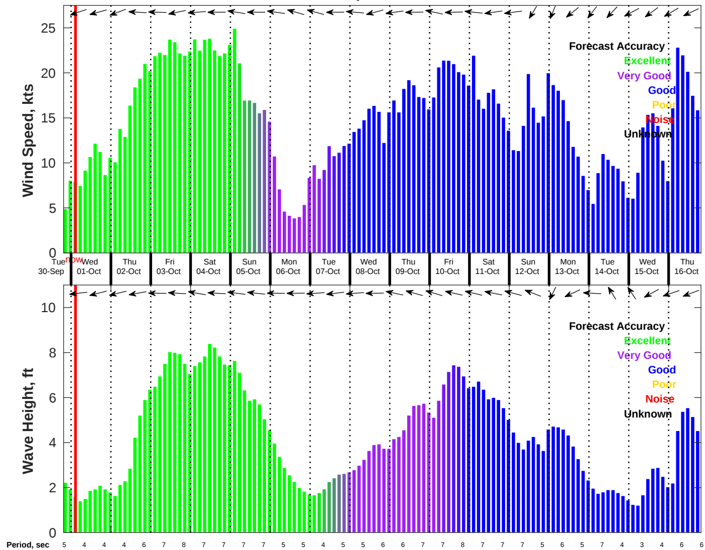
Wind & Wave Forecast for NDBC 42040 from 30-Sep-2025 19:00:00 to 16-Oct-2025 19:00:00
