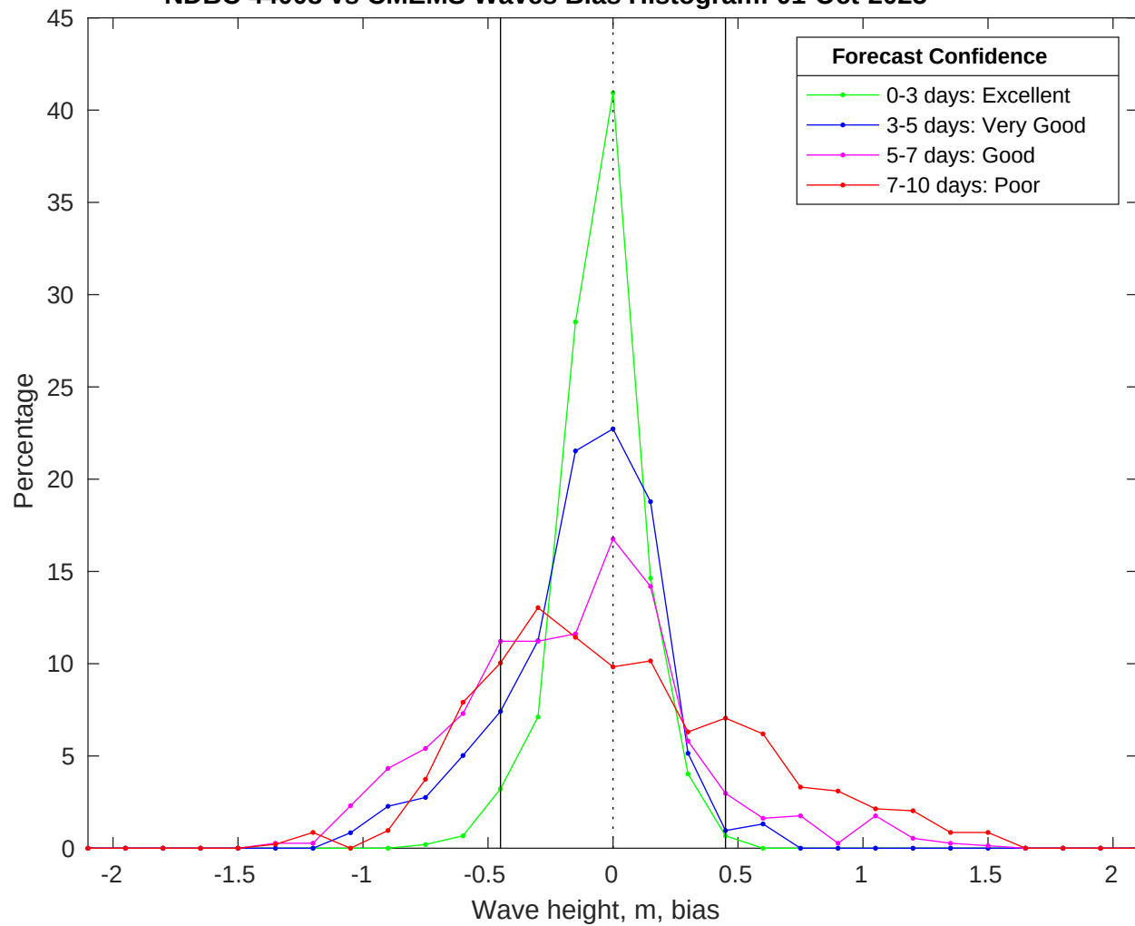
NDBC 44008 vs CMEMS Waves Bias Histogram: 01-Oct-2025
