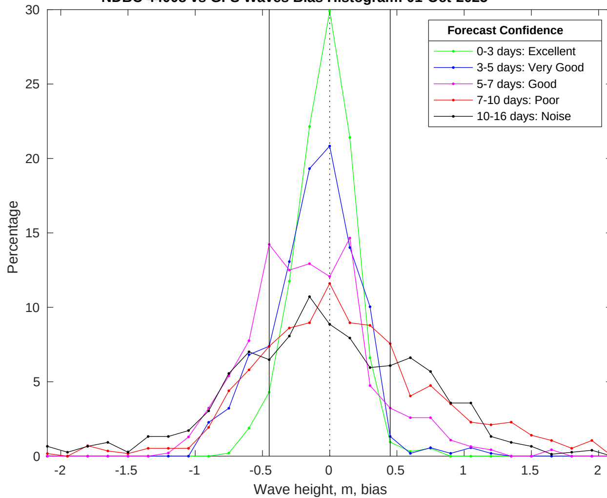
NDBC 44008 vs GFS Waves Bias Histogram: 01-Oct-2025
