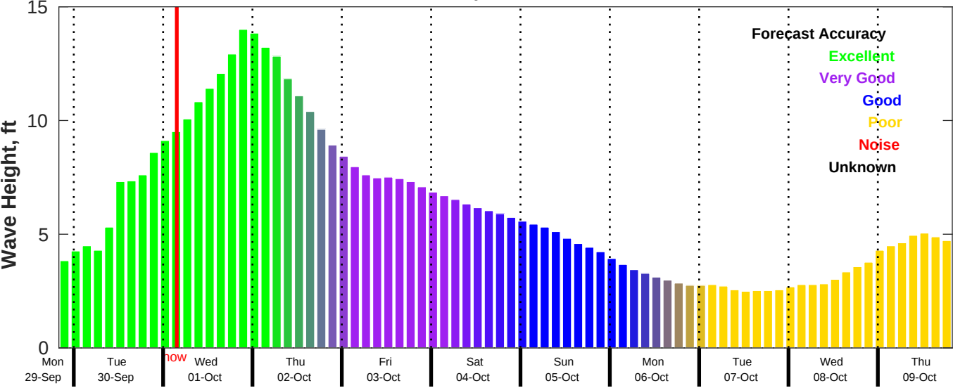
CMEMS Wave Forecast for NDBC 44008 from 29-Sep-2025 20:00:00 to 09-Oct-2025 20:00:00
