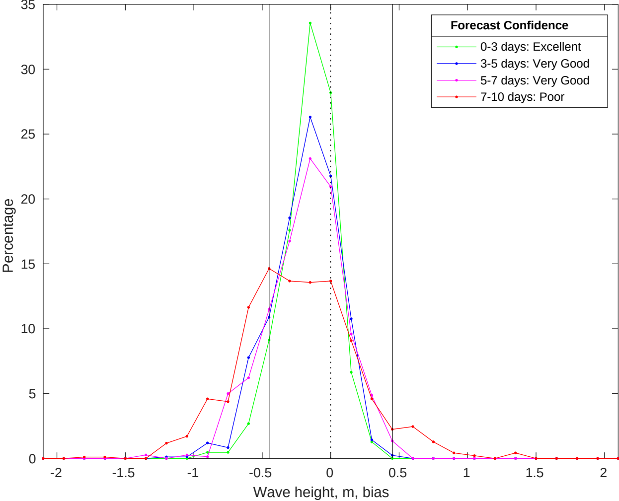
NDBC 46011 vs CMEMS Waves Bias Histogram: 01-Oct-2025
