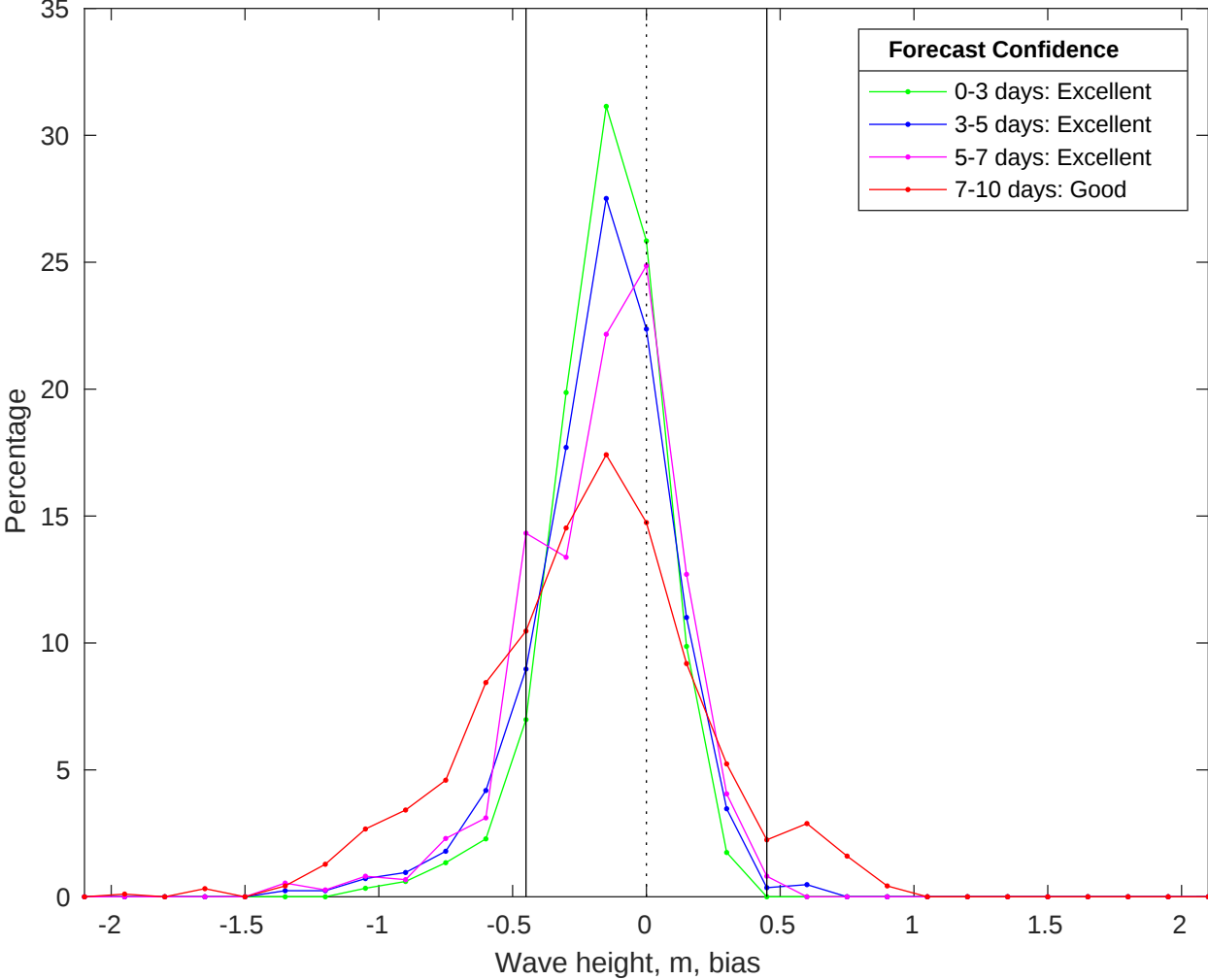
NDBC 46028 vs CMEMS Waves Bias Histogram: 01-Oct-2025
