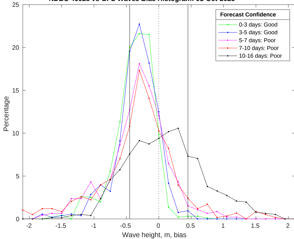
NDBC 46028 vs GFS Waves Bias Histogram: 01-Oct-2025
