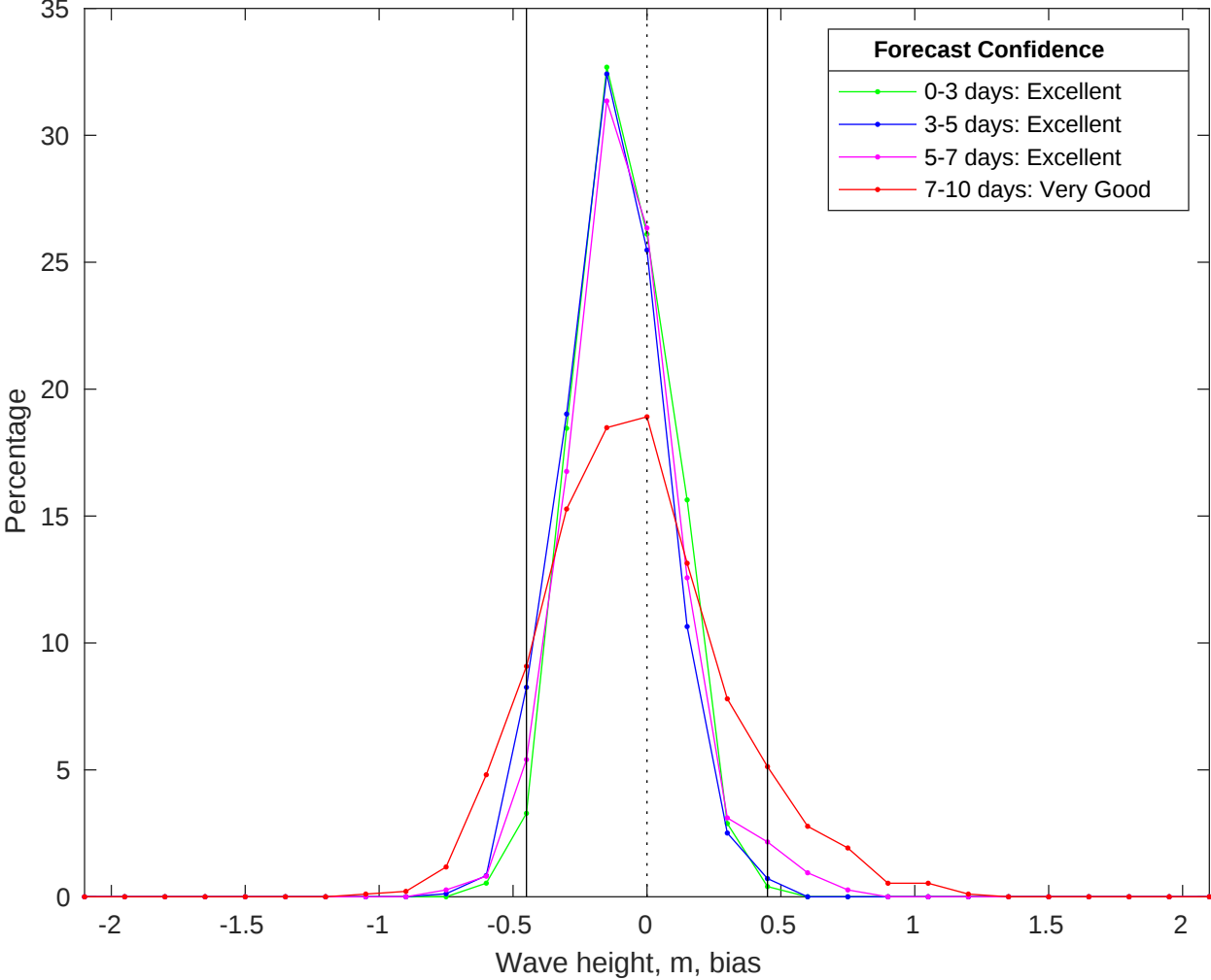
NDBC 46054 vs CMEMS Waves Bias Histogram: 01-Oct-2025
