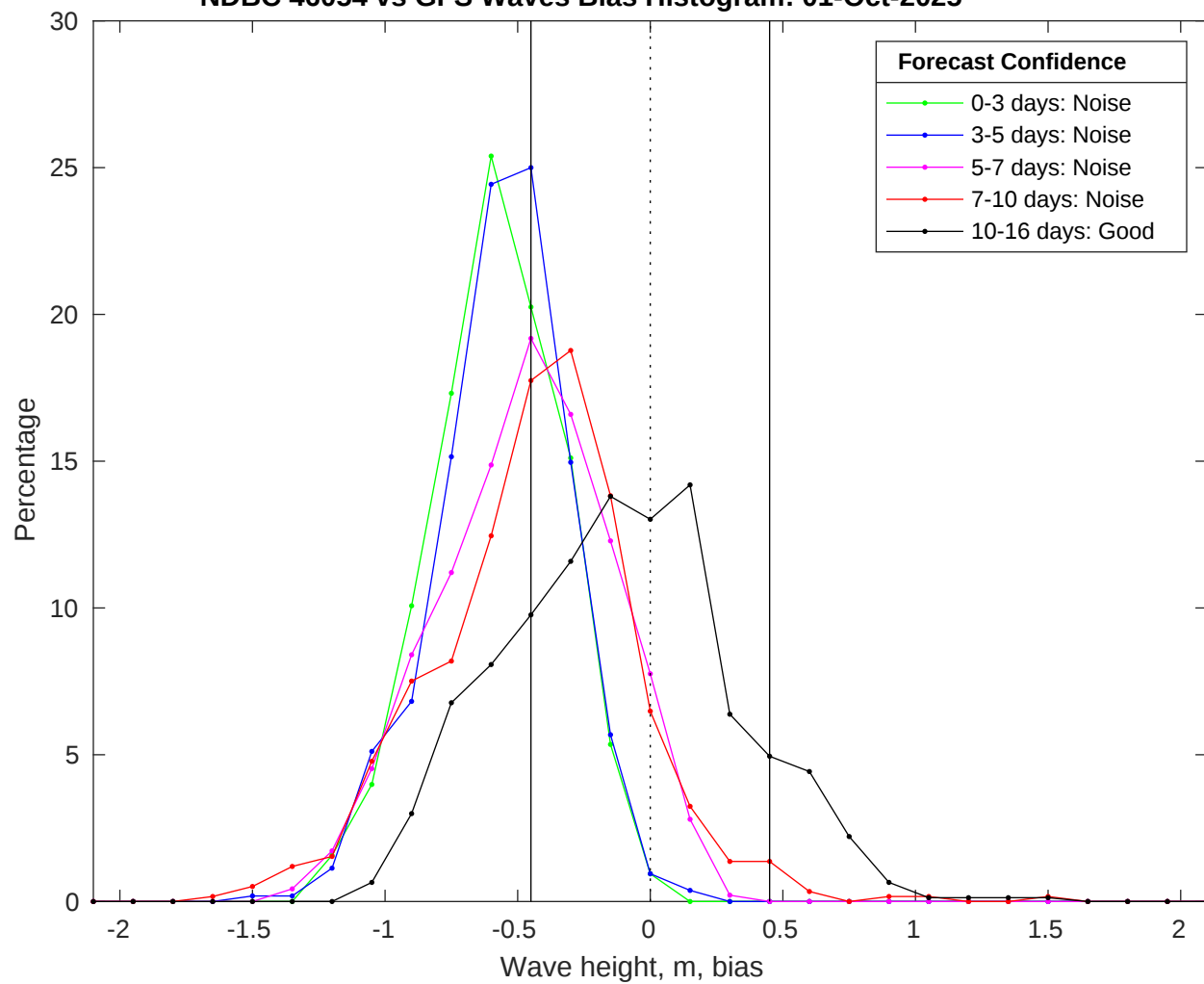
NDBC 46054 vs GFS Waves Bias Histogram: 01-Oct-2025
