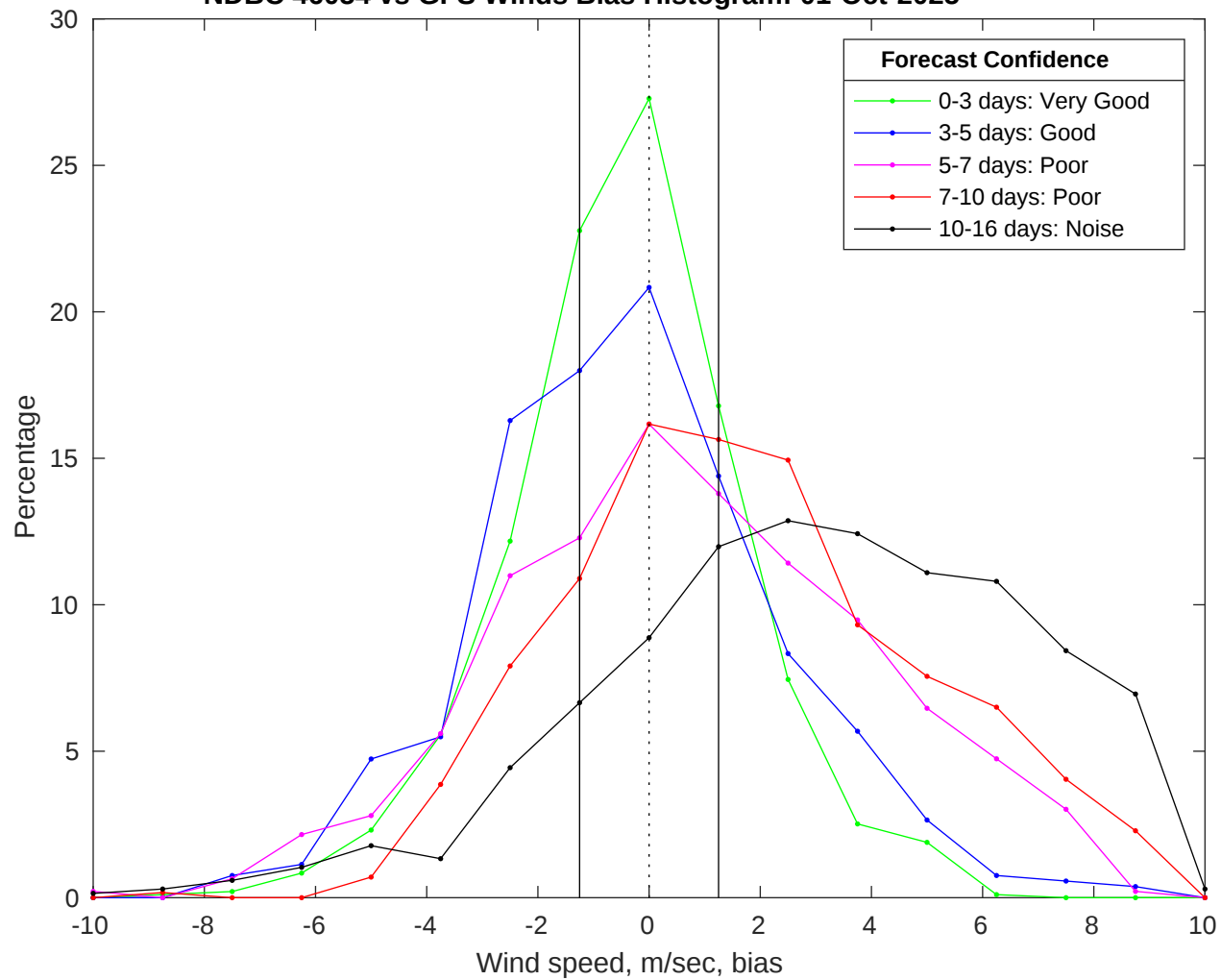
NDBC 46054 vs GFS Winds Bias Histogram: 01-Oct-2025
