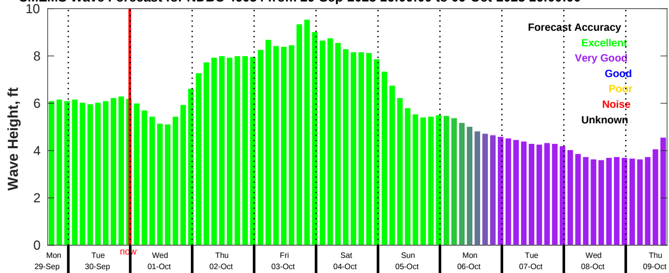
CMEMS Wave Forecast for NDBC 46054 from 29-Sep-2025 16:00:00 to 09-Oct-2025 16:00:00
